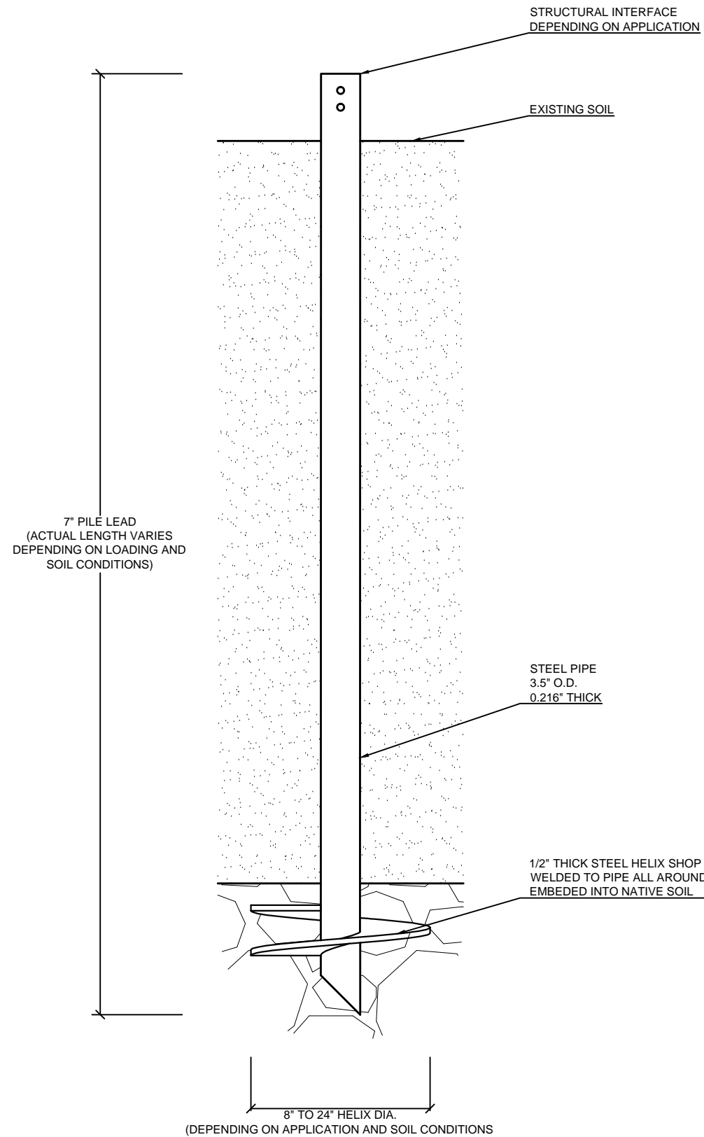
A BCHP3 PILE LEAD - SINGLE HELIX SYSTEM 1"=1'
