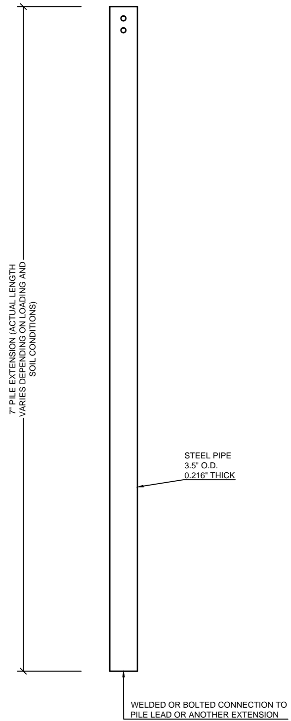
B BCHP3 PILE EXTENSION 1"=1'
