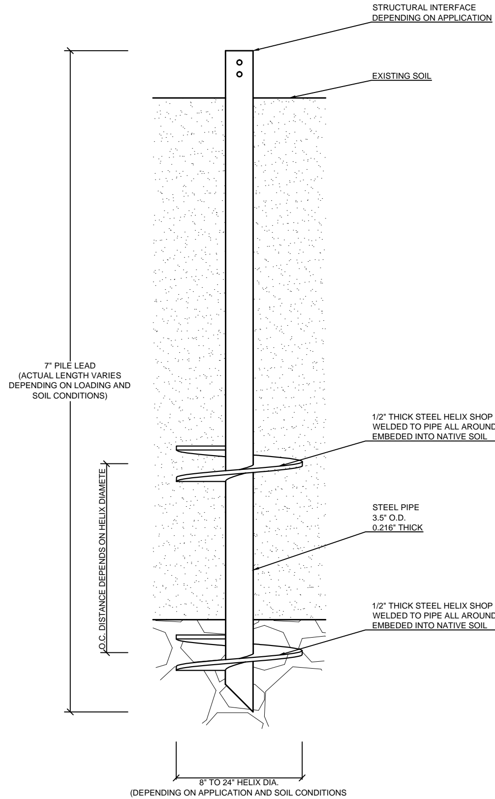
A BCHP3 PILE LEAD - DOUBLE HELIX SYSTEM 1"=1'
