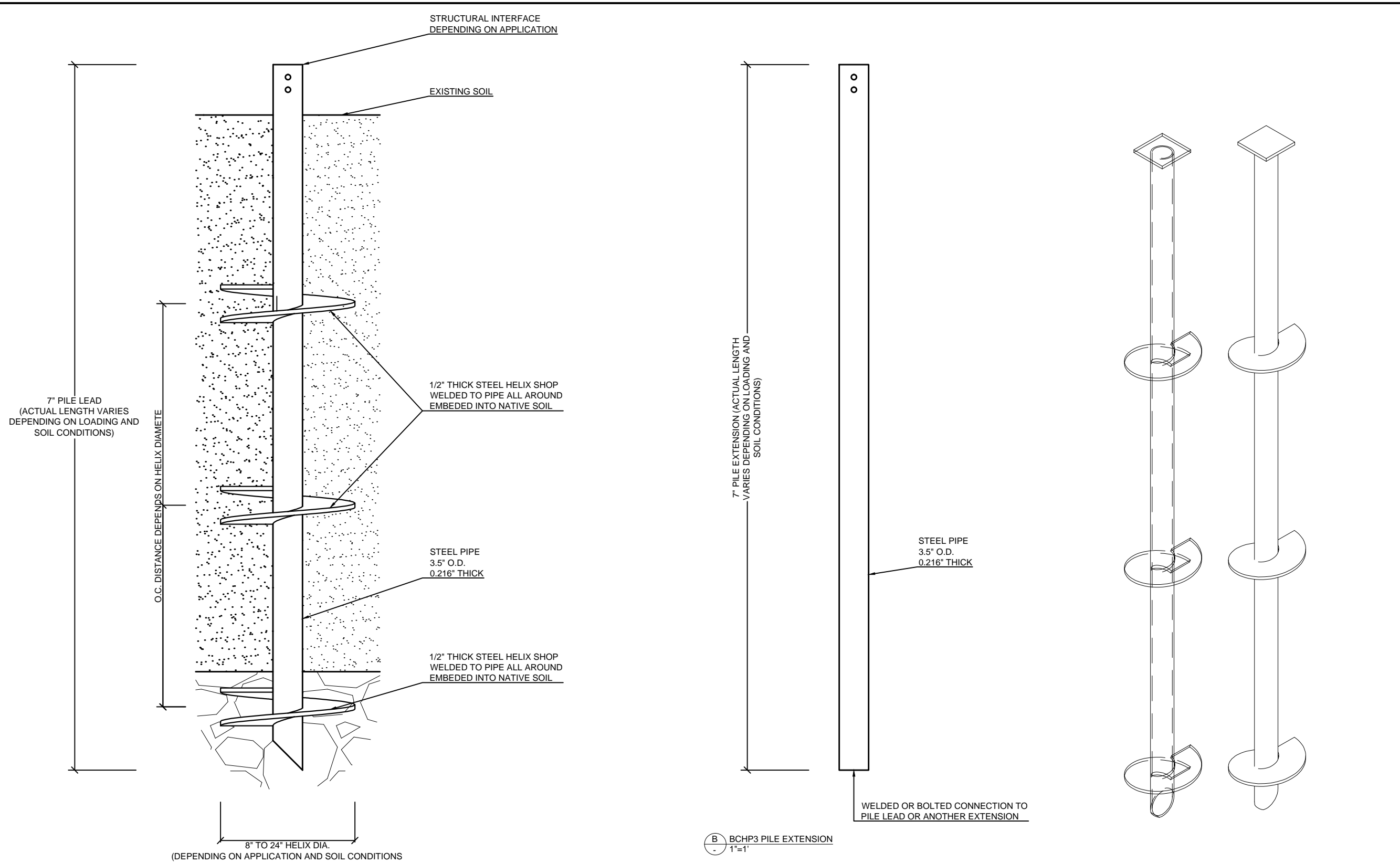
A BCHP3 PILE LEAD - TRIPLE HELIX SYSTEM 1"=1'
