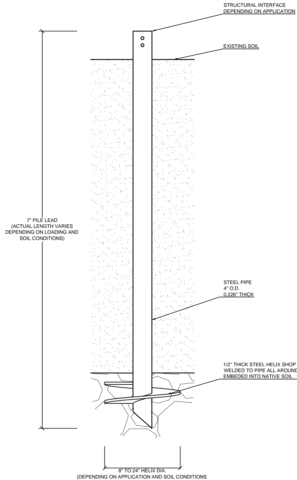
A BCHP4 PILE LEAD - SINGLE HELIX SYSTEM 1"=1'
