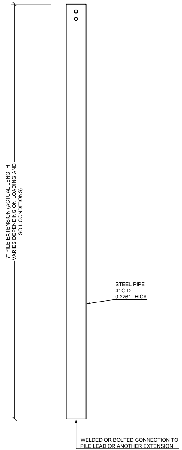
B BCHP4 PILE EXTENSION 1"=1'
