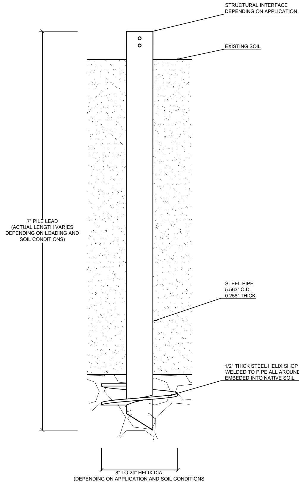
A BCHP5 PILE LEAD - SINGLE HELIX SYSTEM 1"=1'
