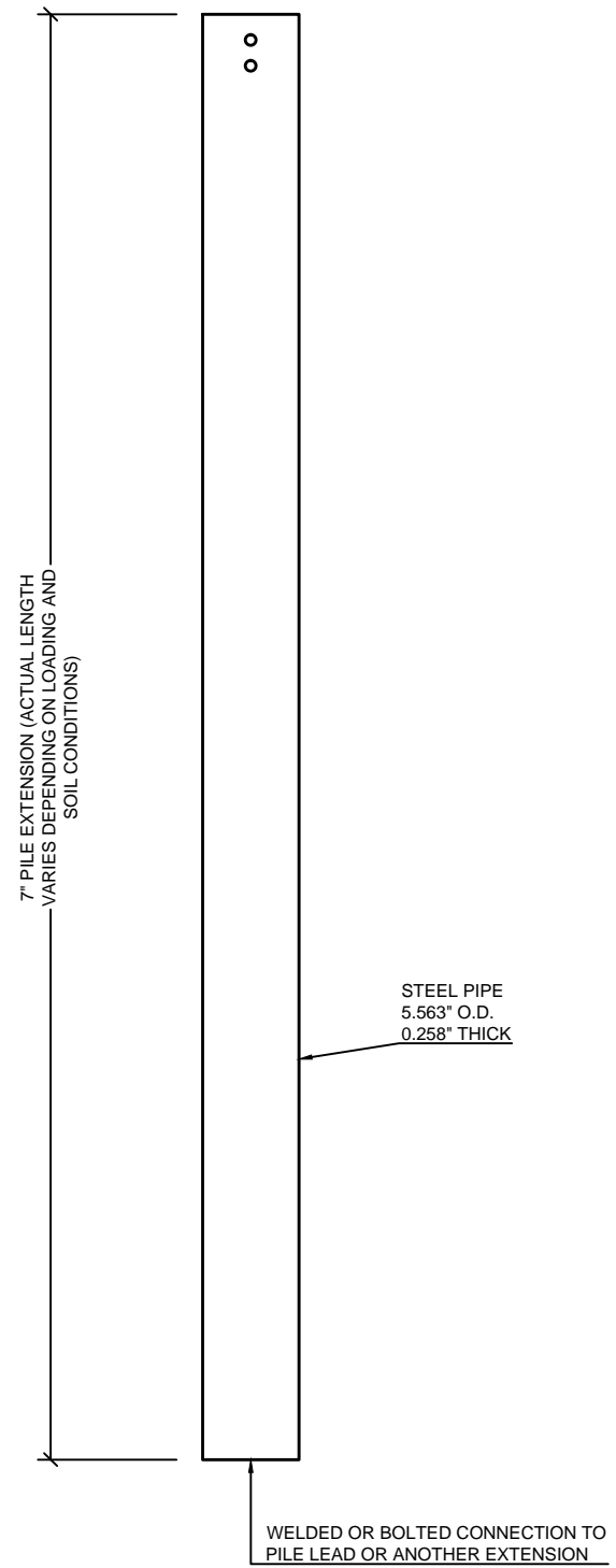
B BCHP5 PILE EXTENSION 1"=1'
